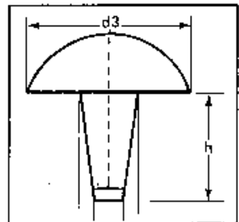
"Drawing of an epidural peg electrode. The electrode is composed of medical grade silicone with a stainless steel or platinum electrode at the base of the stalk."
